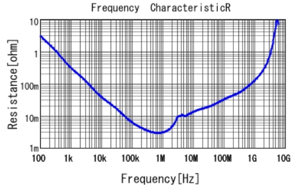
■ GRM21BB30J226ME38 R DCOV, 20degC
