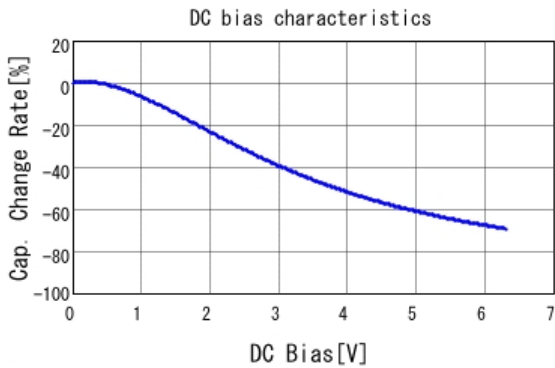
■ GRM21BB30J226ME38 C-DC bias capchange, 20.0degC, AC0.
