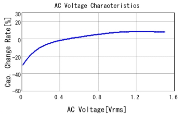
■ GRM21BB30J226ME38 C-AC Voltage capchange, DCOV, 20.0d
