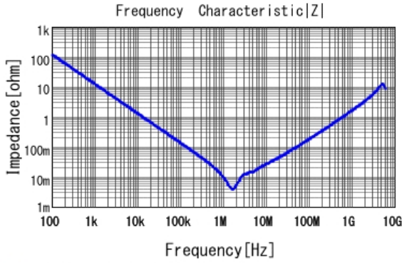
■ GRM21BB30J226ME38 |Z| DCOV, 20degC
