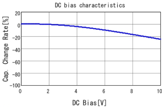
■ GRM21BB11A225KA01 C-DC bias capchange, 20.0degC, AC1.
