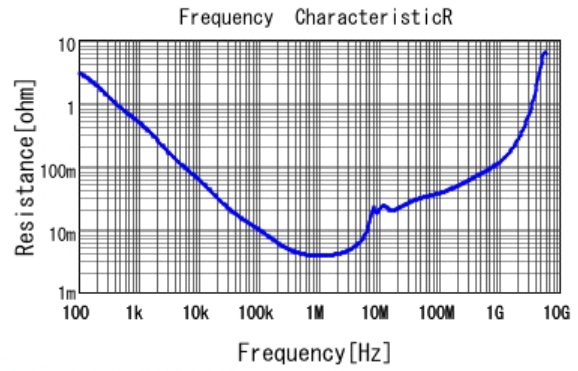
■ GRM21BB11A225KA01 R DCOV, 20degC
