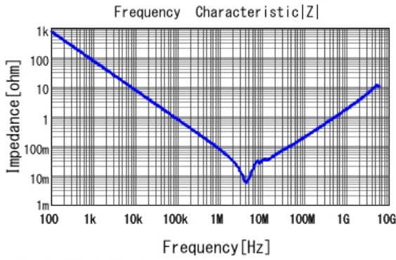
■ GRM21BB11A225KA01 |Z| DCOV, 20degC
