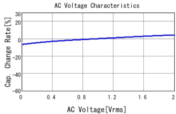
■ GRM21BB11A225KA01 C-AC Voltage capchange, DCOV, 20.0d
