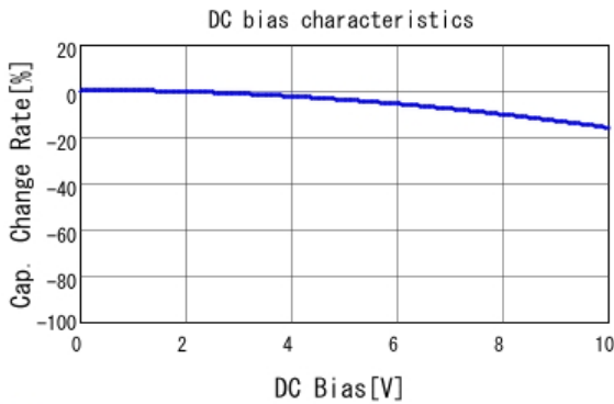
■ GRM21BB11A105KA01 C-DC bias capchange, 20.0degC, AC1.
