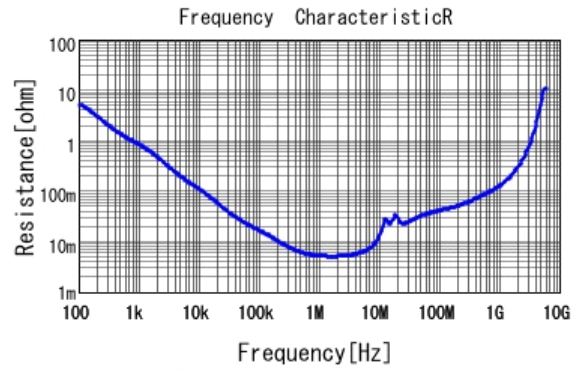
■ GRM21BB11A105KA01 R DCOV, 20degC
