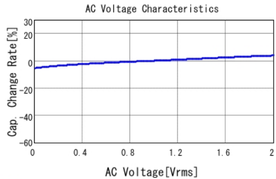
■ GRM21BB11A105KA01 C-AC Voltage capchange, DCOV, 20.0d
