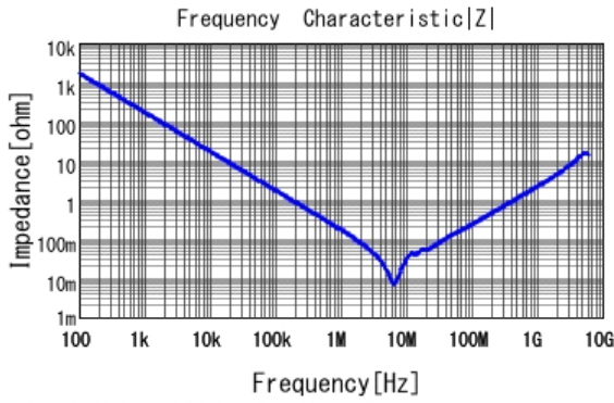
■ GRM21BB11A105KA01 |Z| DCOV, 20degC
