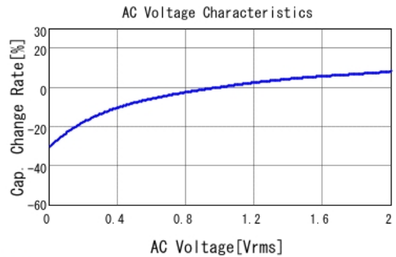
■ GRM21BB10J475KA11 C-AC Voltage capchange, DCOV, 20.0d
