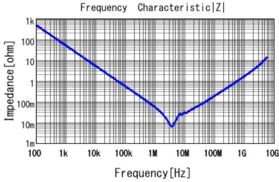
■ GRM21BB10J475KA11 |Z| DCOV, 20degC
