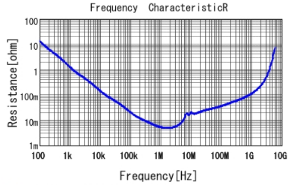
■ GRM21BB10J475KA11 R DCOV, 20degC
