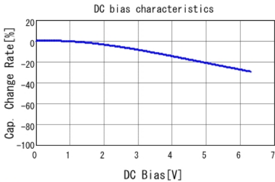
■ GRM21BB10J475KA11 C-DC bias capchange, 20.0degC, AC1.
