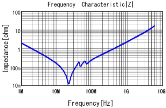
■ GRM21B7U1A823JA01 |Z| DCOV, 25degC
