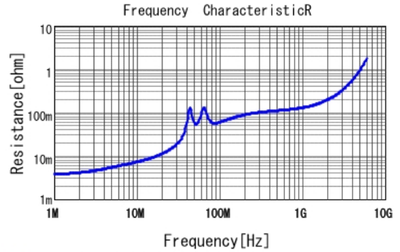
■ GRM21B7U1A823JA01 R DCOV, 25degC
