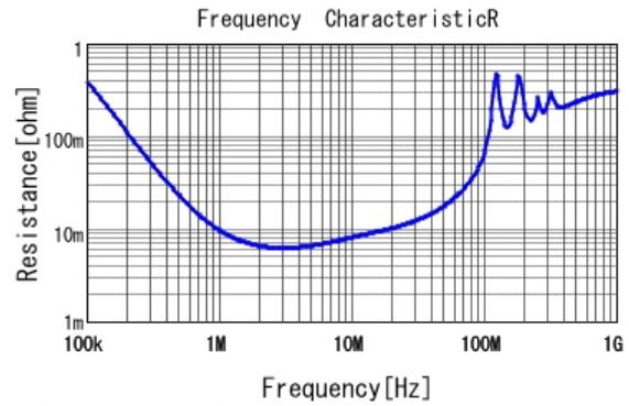
■ GRM21B5C2E103JWAA R DCOV, 25degC
