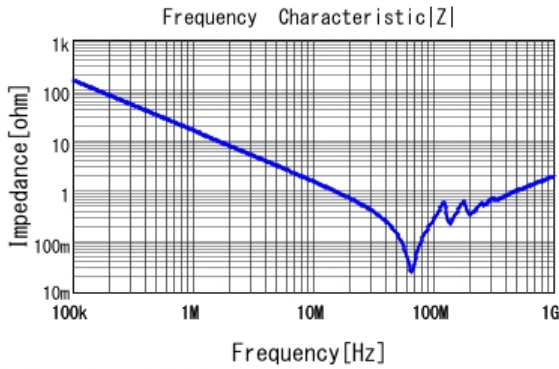
■ GRM21B5C2E103JWAA |Z| DCOV, 25degC
