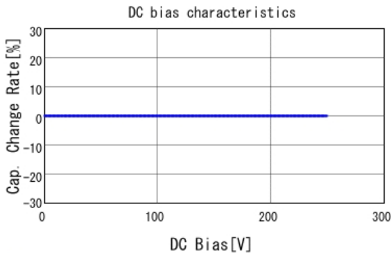
■ GRM21B5C2E103JWAA C-DC bias capchange, 25.0degC, AC1V
