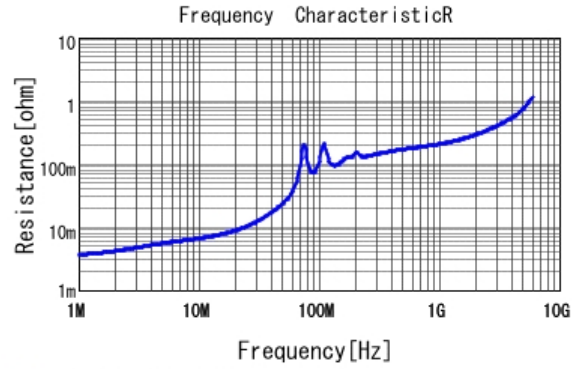
■ GRM21A7U1H333JA39 R DCOV, 25degC
