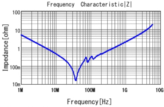
■ GRM21A7U1H333JA39 |Z| DCOV, 25degC
