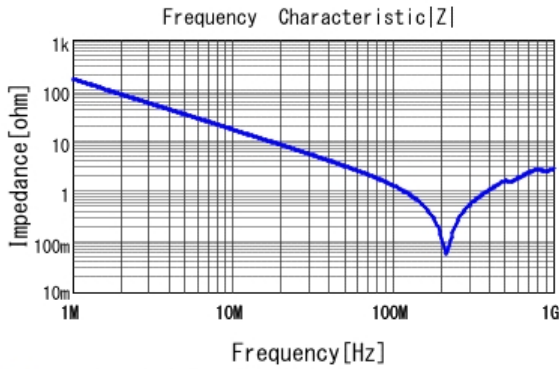
■ GRM21A5C2E102JWA1 |Z| DCOV, 25degC
