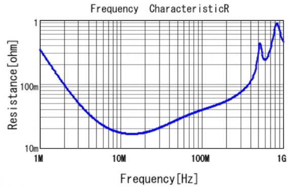
■ GRM21A5C2E102JWA1 R DCOV, 25degC
