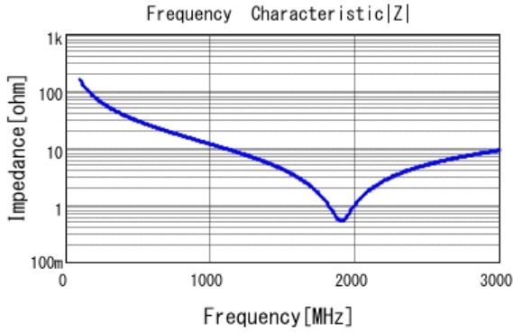
■ GRM21A5C2E100JW01 |Z| DC0V, 25degC
