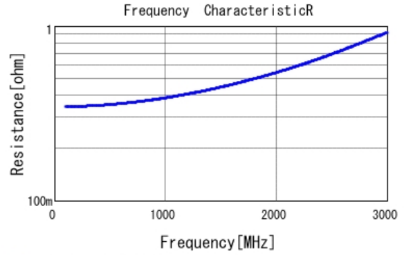
■ GRM21A5C2E100JW01 R DC0V, 25degC
