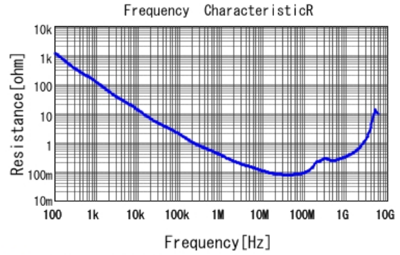
■ GRM219R72A682KA01 R DCOV, 25degC
