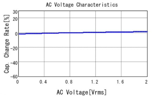
■ GRM219R72A682KA01 C-AC Voltage capchange, DCOV, 25.0d
