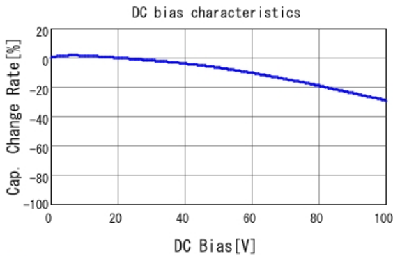
■ GRM219R72A682KA01 C-DC bias capchange, 25.0degC, AC1.
