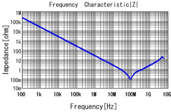
■ GRM219R72A682KA01 |Z| DCOV, 25degC
