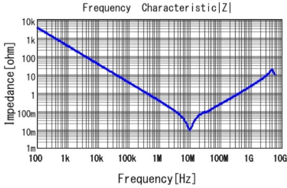
■ GRM219R71C474KA01 |Z| DCOV, 25degC
