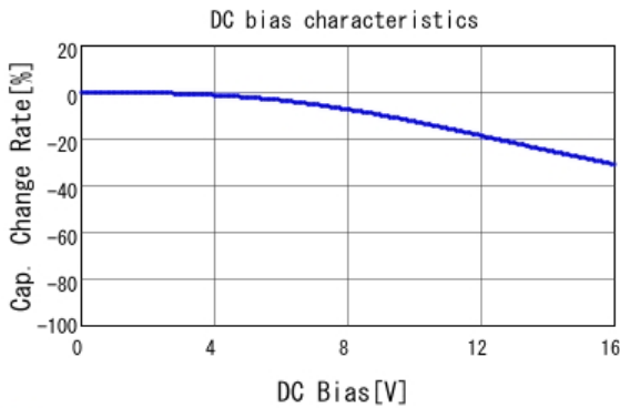
■ GRM219R71C474KA01 C-DC bias capchange, 25.0degC, AC1.
