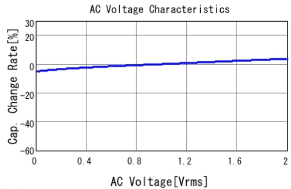
■ GRM219R71C474KA01 C-AC Voltage capchange, DCOV, 25.0d
