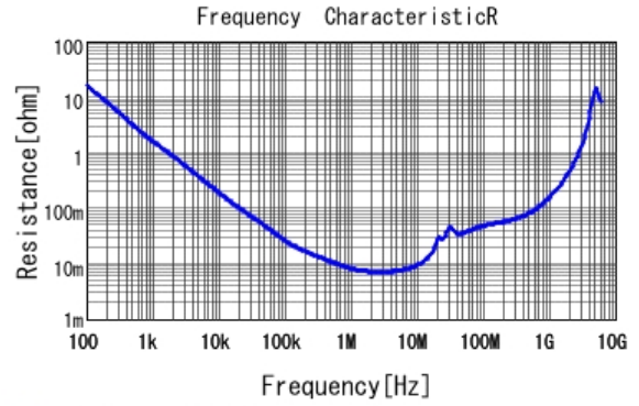
■ GRM219R71C474KA01 R DCOV, 25degC
