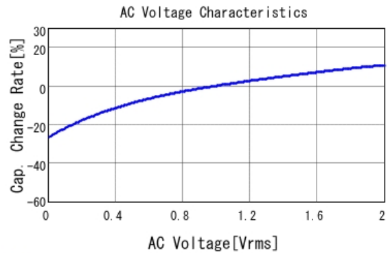
■ GRM219R61H105MA73 C-AC Voltage capchange, DCOV, 25.0d
