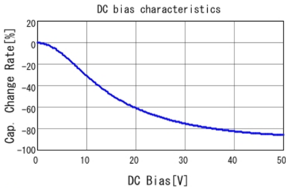
■ GRM219R61H105MA73 C-DC bias capchange, 25.0degC, AC1.
