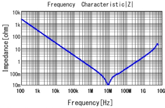
■ GRM219R61H105MA73 |Z| DCOV, 25degC
