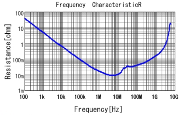
■ GRM219R61H105MA73 R DCOV, 25degC
