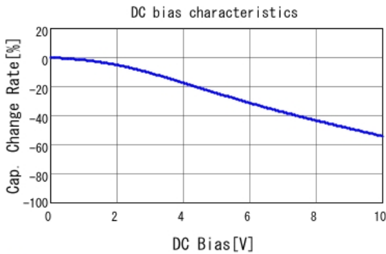
■ GRM219R61A335KE19 C-DC bias capchange, 25.0degC, AC1.
