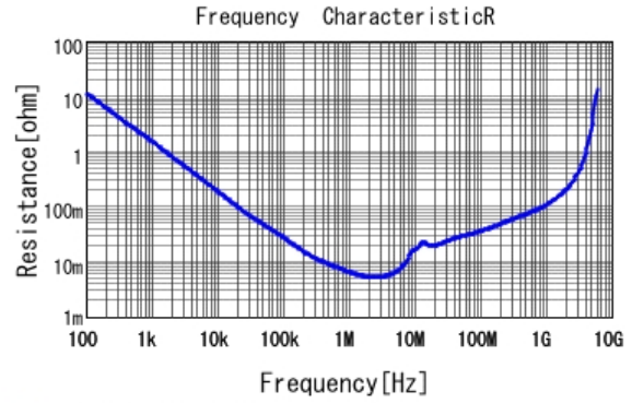
■ GRM219R61A335KE19 R DCOV, 25degC
