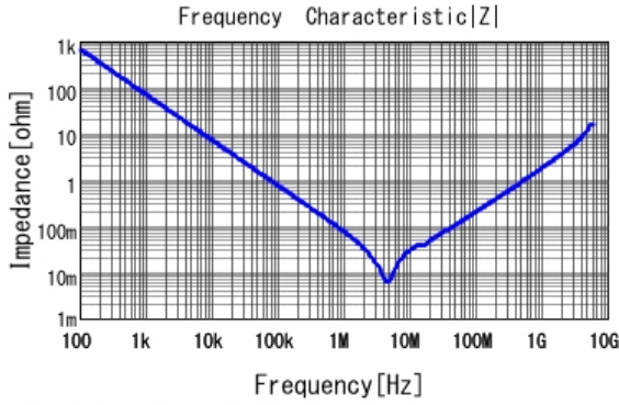
■ GRM219R61A335KE19 |Z| DCOV, 25degC
