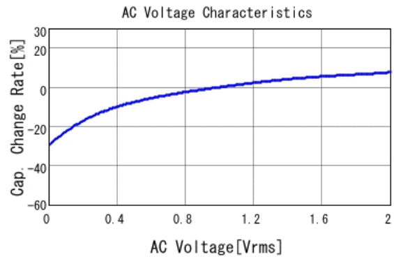
■ GRM219R61A335KE19 C-AC Voltage capchange, DCOV, 25.0d
