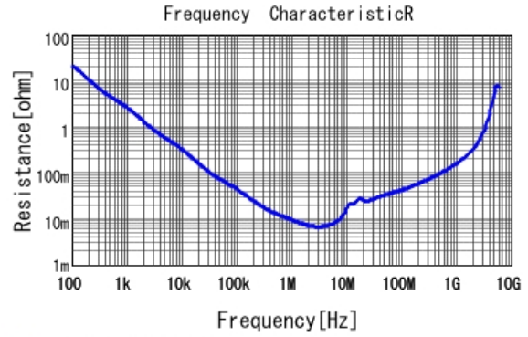
■ GRM219R61A225KA01 R DCOV, 25degC
