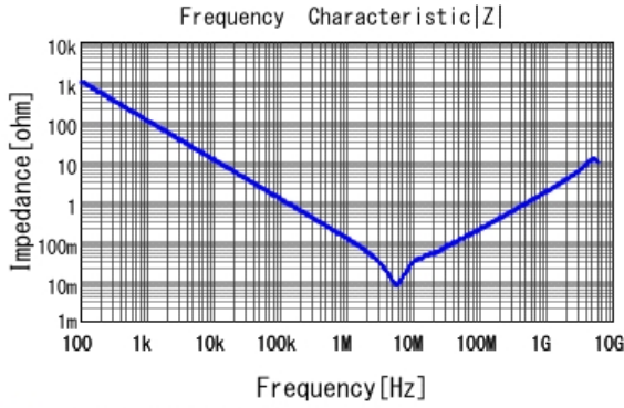
■ GRM219R61A225KA01 |Z| DCOV, 25degC
