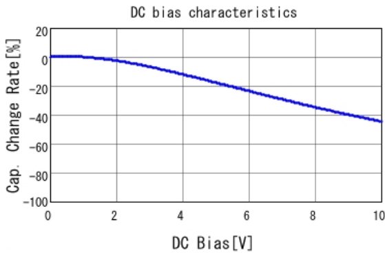
■ GRM219R61A225KA01 C-DC bias capchange, 25.0degC, AC1.
