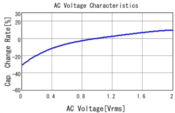
■ GRM219R61A225KA01 C-AC Voltage capchange, DCOV, 25.0d
