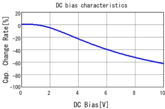
■ GRM219R61A106ME47 C-DC bias capchange, 25.0degC, AC0.
