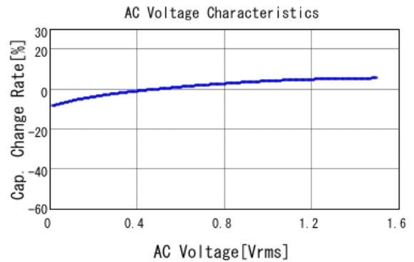
■ GRM219R61A106ME47 C-AC Voltage capchange, DCOV, 25.0d
