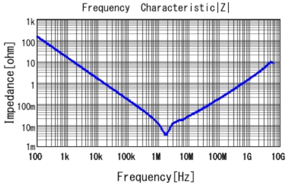
■ GRM219R61A106ME47 |Z| DCOV, 25degC
