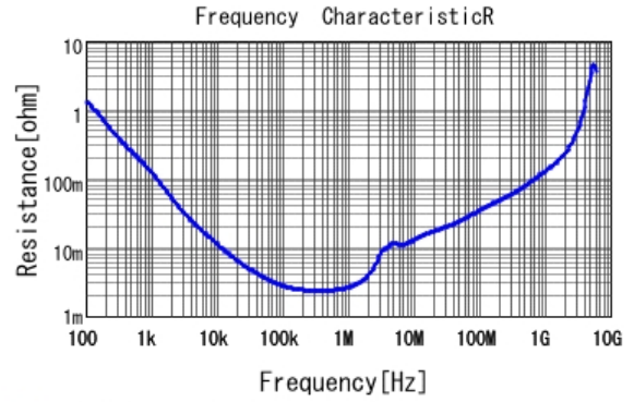
■ GRM219R61A106ME47 R DCOV, 25degC
