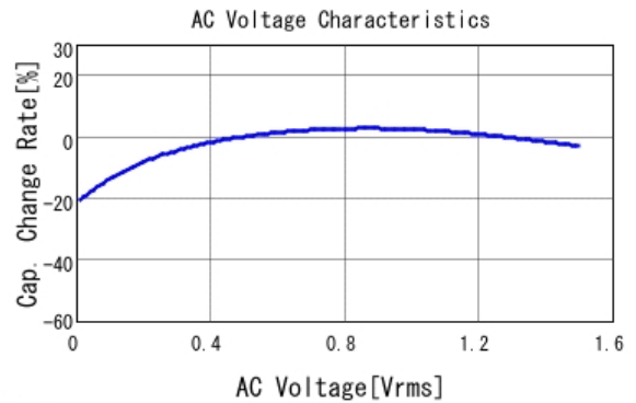
■ GRM219R60J476ME44 C-AC Voltage capchange, DCOV, 25.0d
