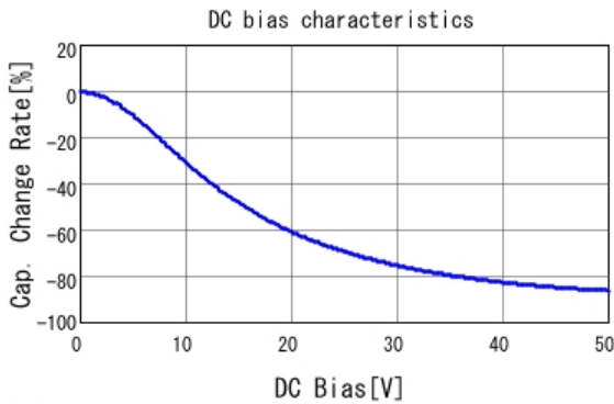
■ GRM219B31H105KA73 C-DC bias capchange, 20.0degC, AC1.
