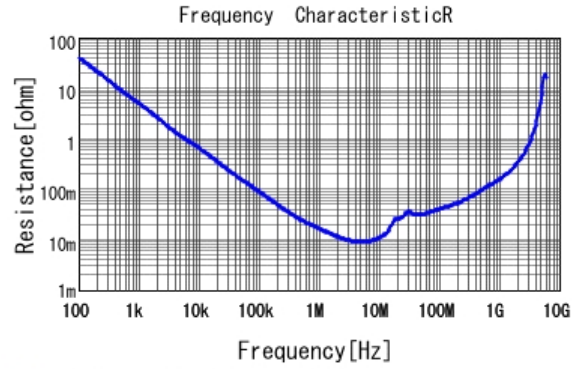
■ GRM219B31H105KA73 R DCOV, 20degC
