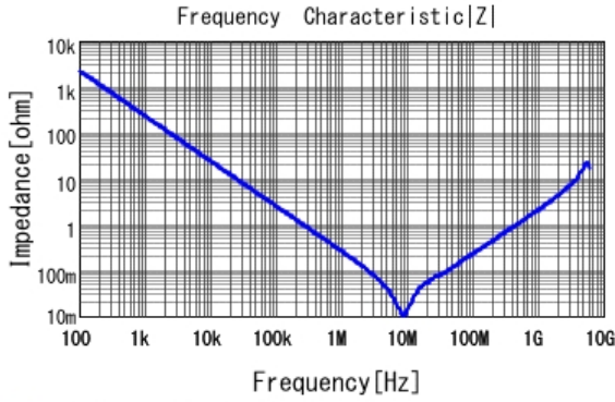
■ GRM219B31H105KA73 |Z| DCOV, 20degC
