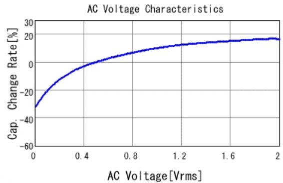
■ GRM219B31C475KE15 C-AC Voltage capchange, DCOV, 20.0d
