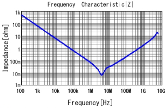
■ GRM219B31C475KE15 |Z| DCOV, 20degC
