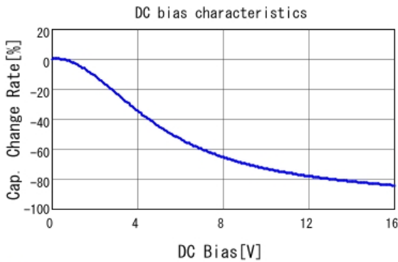
■ GRM219B31C475KE15 C-DC bias capchange, 20.0degC, AC0.
