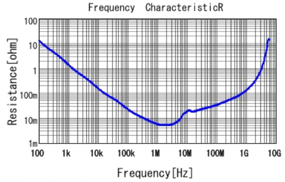
■ GRM219B31C475KE15 R DCOV, 20degC
