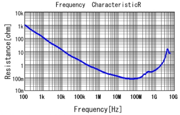
■ GRM216R71H682KA01 R DCOV, 25degC
