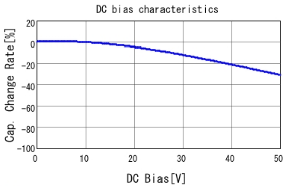
■ GRM216R71H682KA01 C-DC bias capchange, 25.0degC, AC1.
