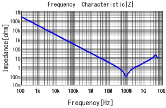
■ GRM216R71H682KA01 |Z| DCOV, 25degC
