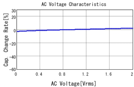
■ GRM216R71H682KA01 C-AC Voltage capchange, DCOV, 25.0d
