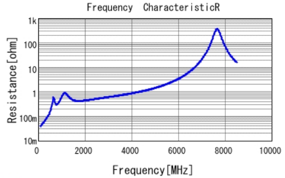
■ GRM2165C2A821JA01 R DCOV, 25degC
