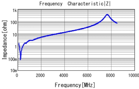
■ GRM2165C2A821JA01 |Z| DCOV, 25degC
