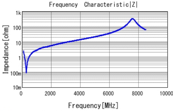
■ GRM2165C2A561JA01 |Z| DCOV, 25degC
