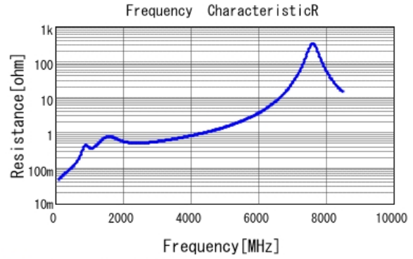
■ GRM2165C2A561JA01 R DCOV, 25degC
