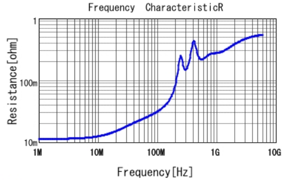
■ GRM2165C2A472JA01 R DCOV, 25degC
