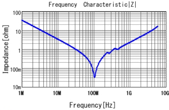
■ GRM2165C2A472JA01 |Z| DCOV, 25degC
