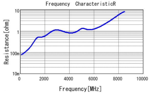
■ GRM2165C2A331JA01 R DCOV, 25degC
