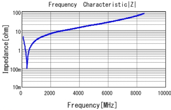
■ GRM2165C2A331JA01 |Z| DCOV, 25degC
