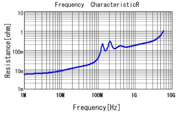
■ GRM2165C2A153JA01 R DCOV, 25degC
