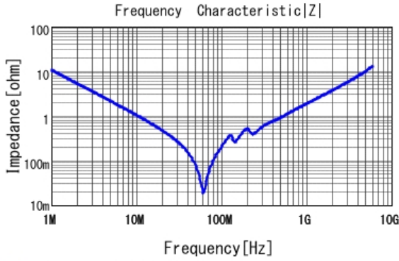
■ GRM2165C2A153JA01 |Z| DCOV, 25degC
