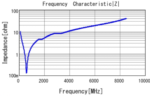
■ GRM2165C2A151JA01 |Z| DCOV, 25degC
