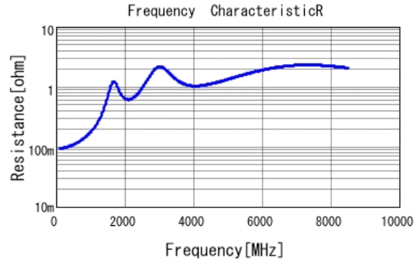
■ GRM2165C2A151JA01 R DCOV, 25degC
