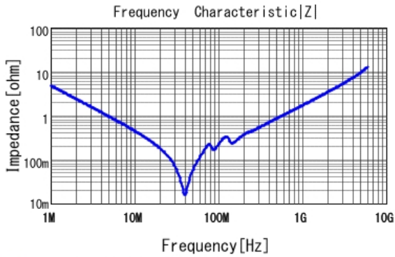
■ GRM2165C1H333JA01 |Z| DCOV, 25degC
