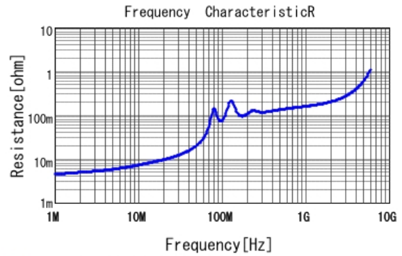
■ GRM2165C1H333JA01 R DCOV, 25degC
