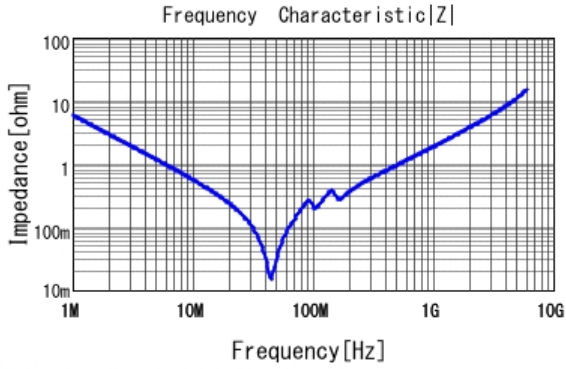
■ GRM2165C1H273JA01 |Z| DCOV, 25degC
