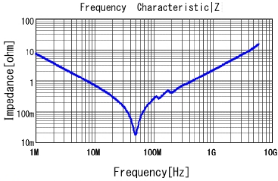
■ GRM2165C1H223JA01 |Z| DCOV, 25degC
