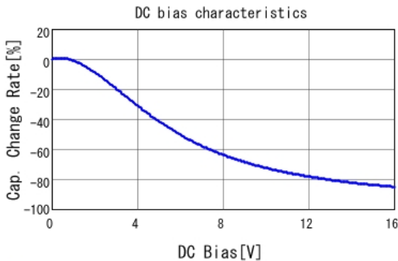
■ GRM188Z71C475ME21 C-DC bias capchange, 25.0degC, AC1V
