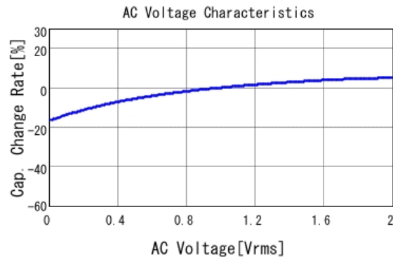
■ GRM188Z71C475ME21 C-AC Voltage capchange, DCOV, 25.0d
