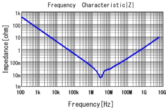
■ GRM188Z71C475ME21 |Z| DCOV, 25degC
