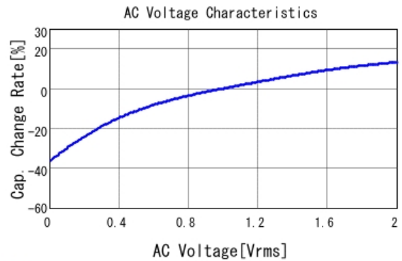
■ GRM188R7YA105MA12 C-AC Voltage capchange, DCOV, 25.0d
