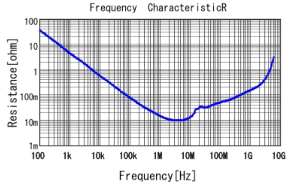
■ GRM188R7YA105MA12 R DCOV, 25degC
