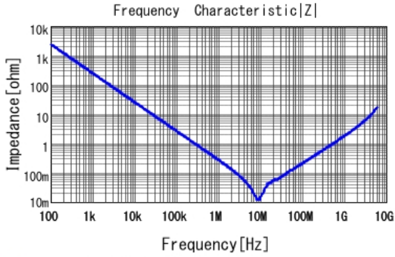
■ GRM188R7YA105MA12 |Z| DCOV, 25degC
