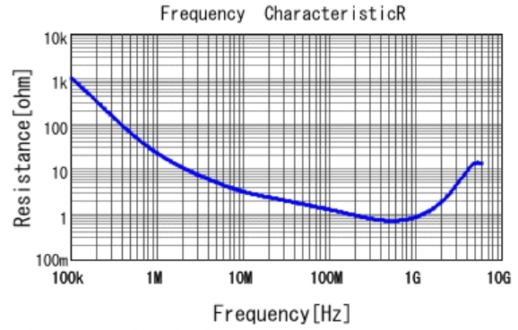
■ GRM188R72E221KW07 R DCOV, 25degC
