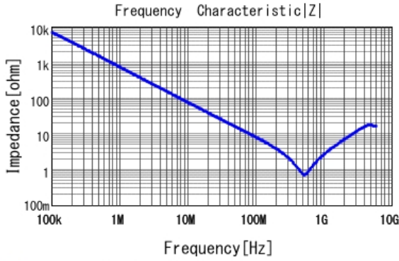
■ GRM188R72E221KW07 |Z| DCOV, 25degC
