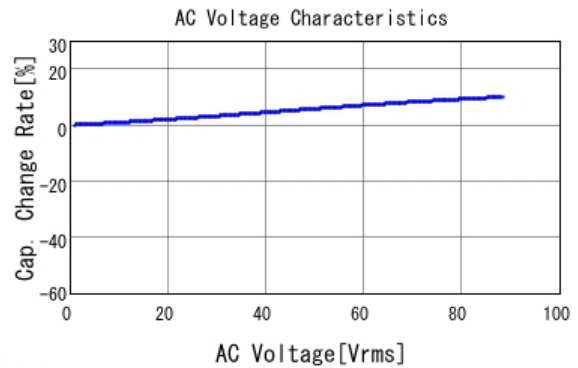
■ GRM188R72E221KW07 C-AC Voltage capchange, DCOV, 25.0d
