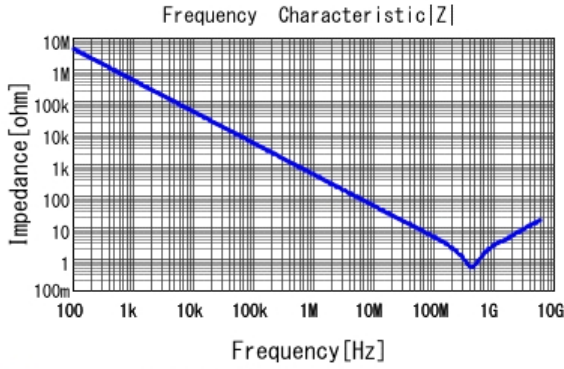
■ GRM188R72A331KA01 |Z| DCOV, 25degC
