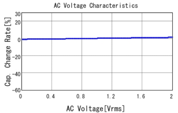
■ GRM188R72A331KA01 C-AC Voltage capchange, DCOV, 25.0d
