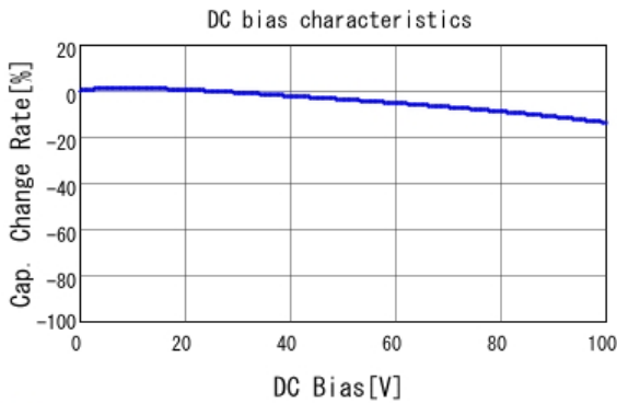
■ GRM188R72A331KA01 C-DC bias capchange, 25.0degC, AC1.
