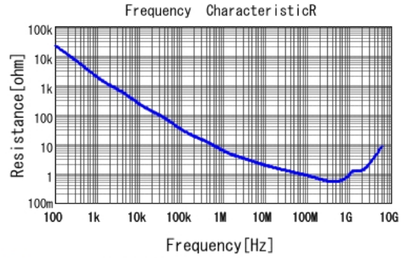
■ GRM188R72A331KA01 R DCOV, 25degC
