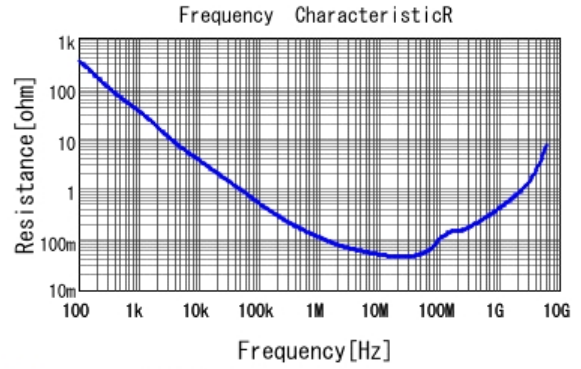
■ GRM188R72A223KAC4 R DCOV, 25degC
