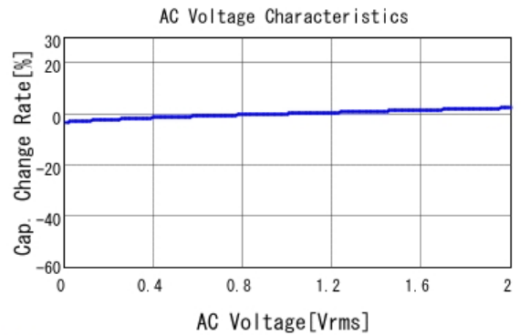
■ GRM188R72A223KAC4 C-AC Voltage capchange, DCOV, 25.0d
