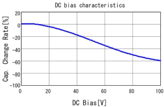
■ GRM188R72A153KAC4 C-DC bias capchange, 25.0degC, AC1.
