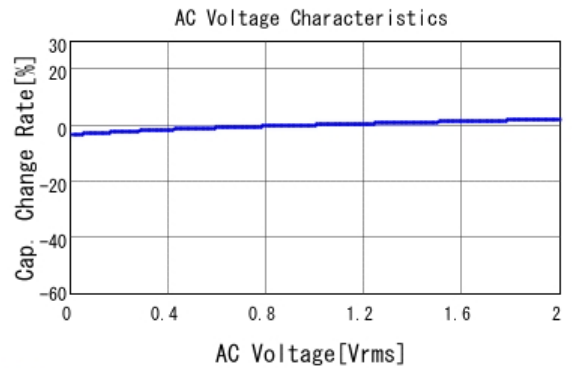
■ GRM188R72A153KAC4 C-AC Voltage capchange, DCOV, 25.0d
