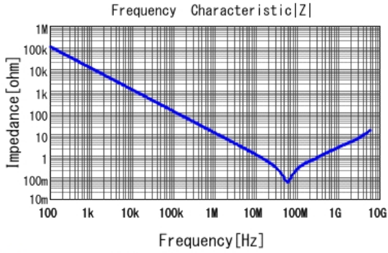
■ GRM188R72A153KAC4 |Z| DCOV, 25degC
