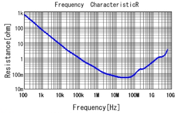
■ GRM188R72A153KAC4 R DCOV, 25degC
