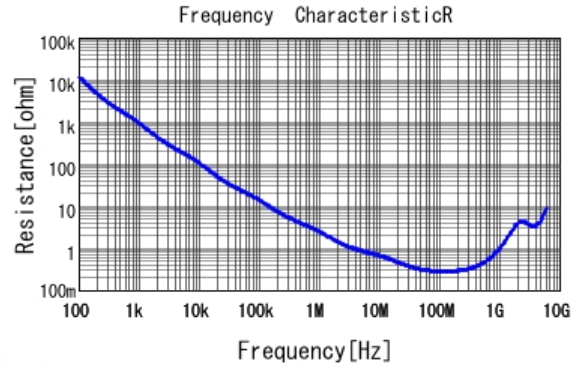
■ GRM188R72A102MA01 R DCOV, 25degC
