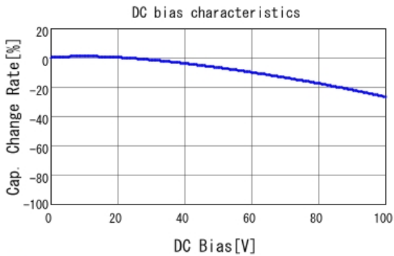
■ GRM188R72A102MA01 C-DC bias capchange, 25.0degC, AC1.
