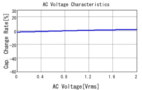
■ GRM188R72A102MA01 C-AC Voltage capchange, DCOV, 25.0d
