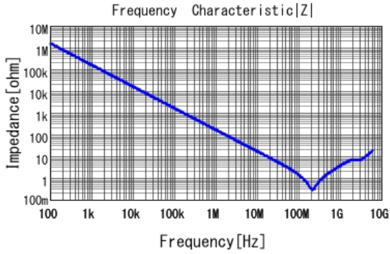
■ GRM188R72A102MA01 |Z| DCOV, 25degC
