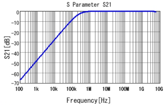
■ GRM188R71H682KA01 S21 DC0V, 25degC
