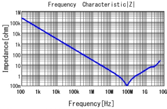
■ GRM188R71H682KA01 |Z| DCOV, 25degC
