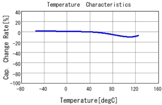
■ GRM188R71H682KA01 C-Temp. capchange, DC0.0V, AC1.0V rm
