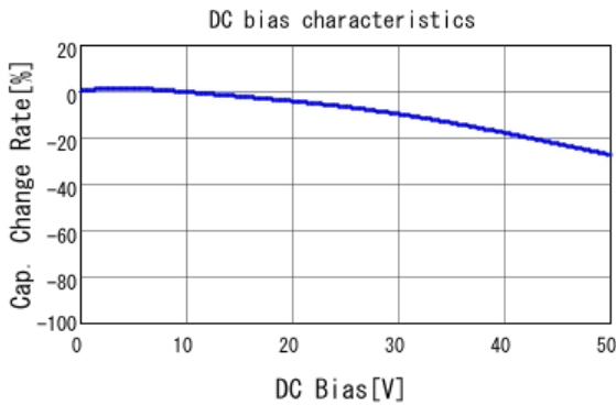
■ GRM188R71H682KA01 C-DC bias capchange, 25.0degC, AC1.
