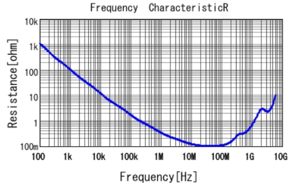
■ GRM188R71H682KA01 R DCOV, 25degC
