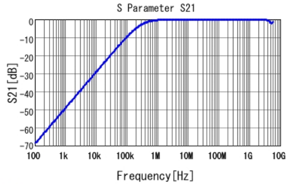
■ GRM188R71H562KA01 S21 DC0V, 25degC
