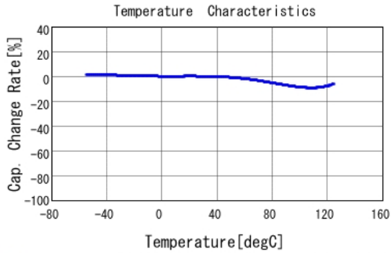
■ GRM188R71H562KA01 C-Temp. capchange, DC0.0V, AC1.0V rm
