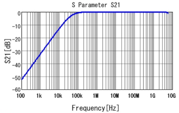
■ GRM188R71H393KA61 S21 DC0V, 25degC
