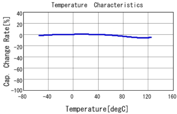
■ GRM188R71H393KA61 C-Temp. capchange, DC0.0V, AC1.0V rm
