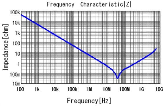
■ GRM188R71H393KA61 |Z| DCOV, 25degC
