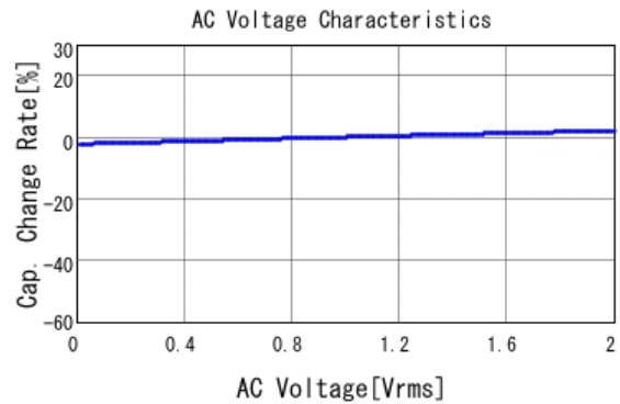
■ GRM188R71H393KA61 C-AC Voltage capchange, DCOV, 25.0d
