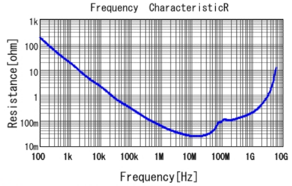
■ GRM188R71H393KA61 R DCOV, 25degC
