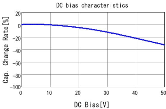
■ GRM188R71H393KA61 C-DC bias capchange, 25.0degC, AC1.
