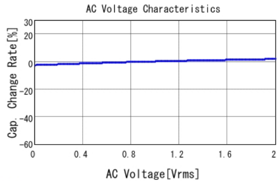
■ GRM188R71H392KA01 C-AC Voltage capchange, DCOV, 25.0d
