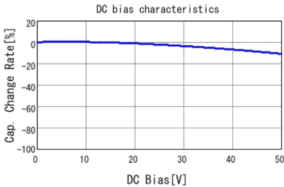
■ GRM188R71H392KA01 C-DC bias capchange, 25.0degC, AC1.
