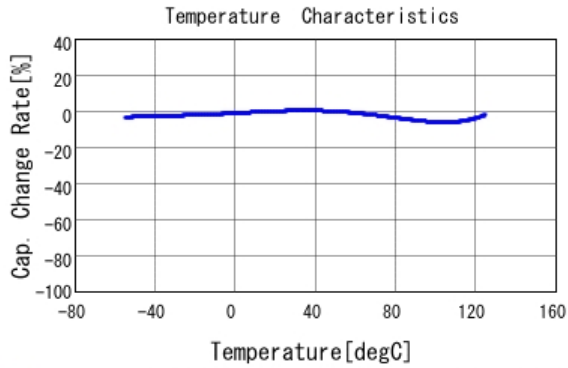
■ GRM188R71H392KA01 C-Temp. capchange, DC0.0V, AC1.0Vrm
