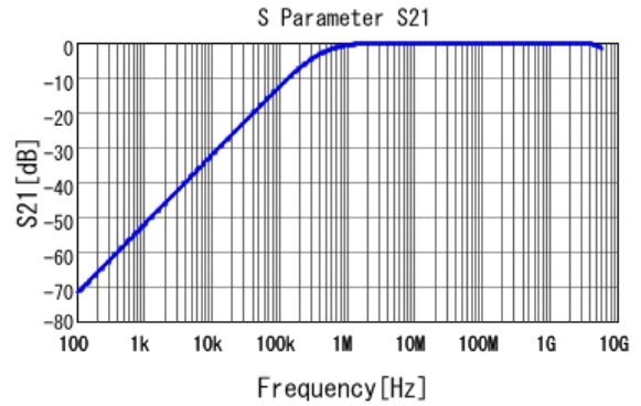
■ GRM188R71H392KA01 S21 DC0V, 25degC
