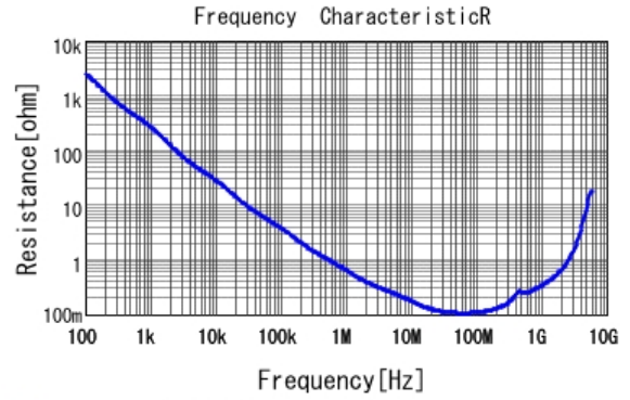
■ GRM188R71H392KA01 R DCOV, 25degC
