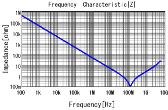
■ GRM188R71H392KA01 |Z| DCOV, 25degC
