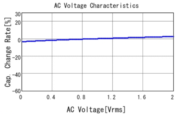
■ GRM188R71H224KAC4 C-AC Voltage capchange, DCOV, 25.0d
