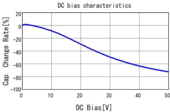
■ GRM188R71H224KAC4 C-DC bias capchange, 25.0degC, AC1.
