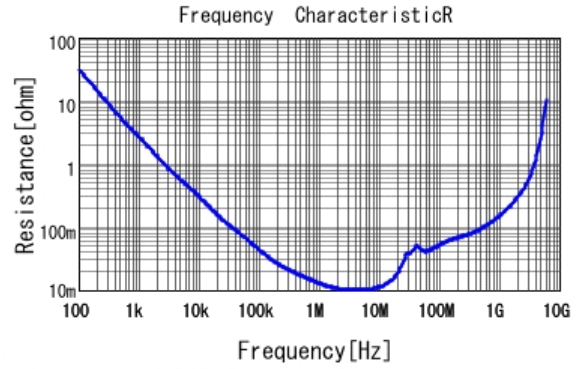
■ GRM188R71H224KAC4 R DCOV, 25degC
