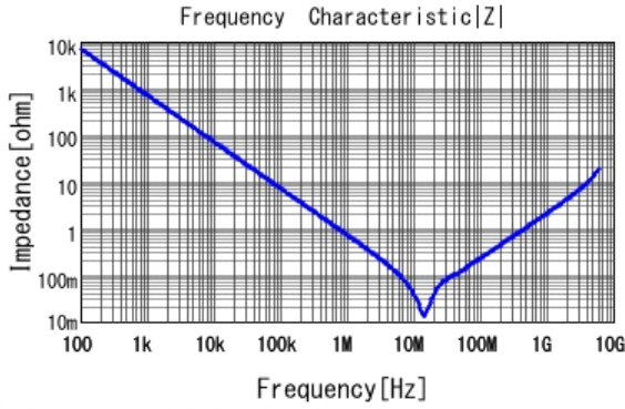
■ GRM188R71H224KAC4 |Z| DCOV, 25degC
