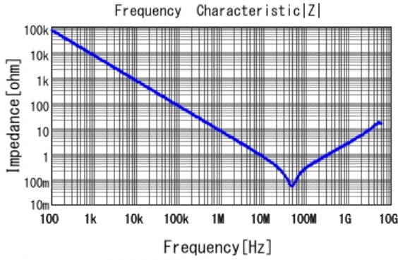
■ GRM188R71H223MA01 |Z| DCOV, 25degC
