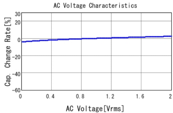
■ GRM188R71H223MA01 C-AC Voltage capchange, DCOV, 25.0d
