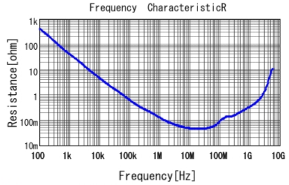
■ GRM188R71H223MA01 R DCOV, 25degC
