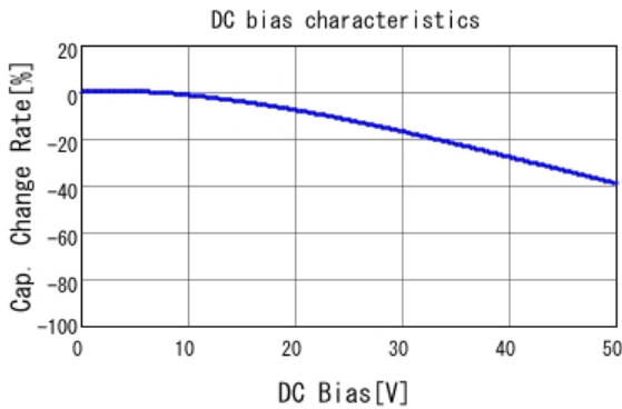
■ GRM188R71H223MA01 C-DC bias capchange, 25.0degC, AC1.
