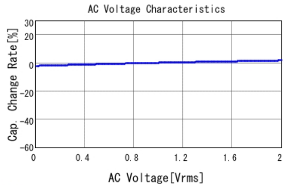
■ GRM188R71H123KA01 C-AC Voltage capchange, DCOV, 25.0d
