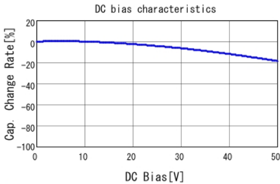
■ GRM188R71H123KA01 C-DC bias capchange, 25.0degC, AC1.
