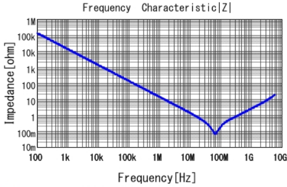
■ GRM188R71H123KA01 |Z| DCOV, 25degC
