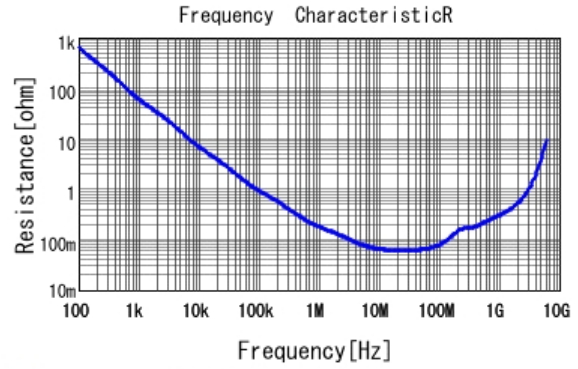
■ GRM188R71H123KA01 R DCOV, 25degC
