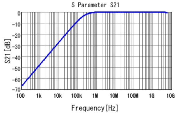
■ GRM188R71E682KA01 S21 DC0V, 25degC
