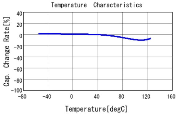
■ GRM188R71E682KA01 C-Temp. capchange, DC0.0V, AC1.0Vrm
