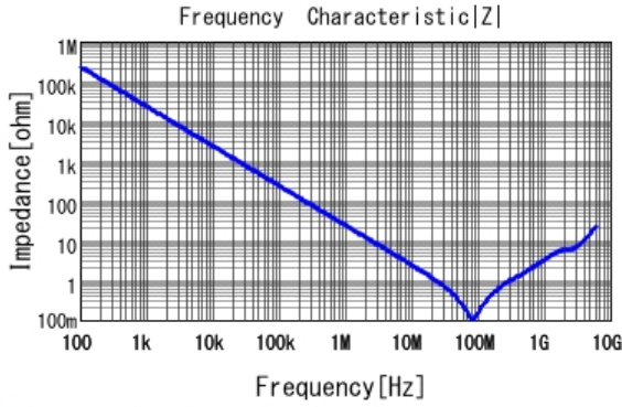
■ GRM188R71E682KA01 |Z| DCOV, 25degC
