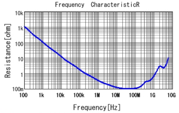
■ GRM188R71E682KA01 R DCOV, 25degC
