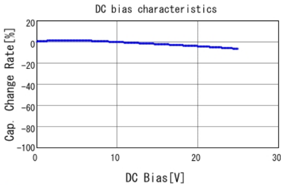
■ GRM188R71E682KA01 C-DC bias capchange, 25.0degC, AC1.
