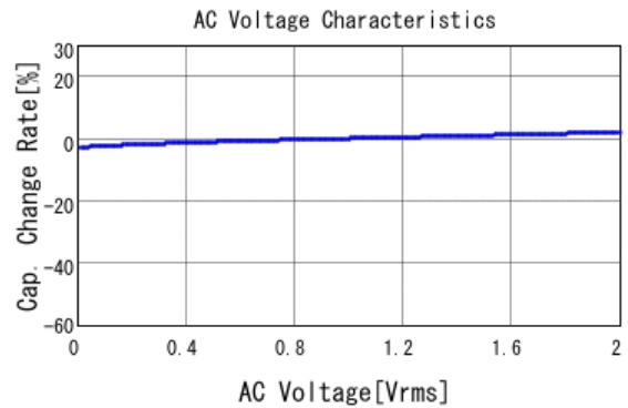
■ GRM188R71E682KA01 C-AC Voltage capchange, DCOV, 25.0d
