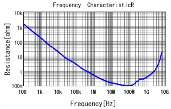
■ GRM188R71E472KA01 R DCOV, 25degC
