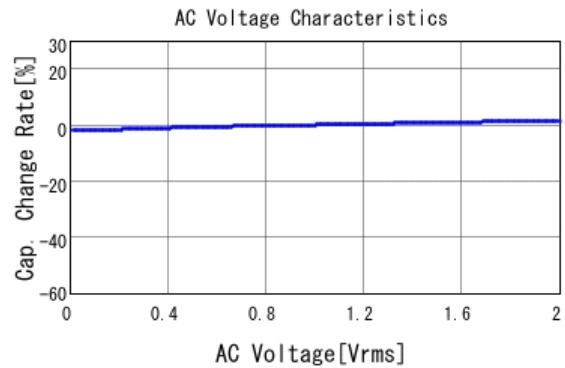
■ GRM188R71E472KA01 C-AC Voltage capchange, DCOV, 25.0d
