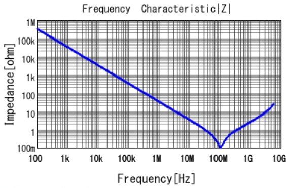
■ GRM188R71E472KA01 |Z| DCOV, 25degC
