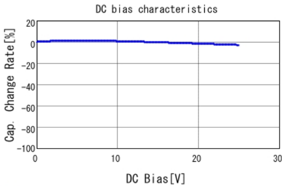
■ GRM188R71E472KA01 C-DC bias capchange, 25.0degC, AC1.
