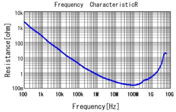
■ GRM188R71E332KA01 R DCOV, 25degC
