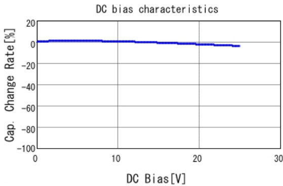
■ GRM188R71E332KA01 C-DC bias capchange, 25.0degC, AC1.
