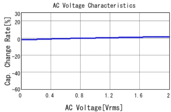
■ GRM188R71E332KA01 C-AC Voltage capchange, DCOV, 25.0d
