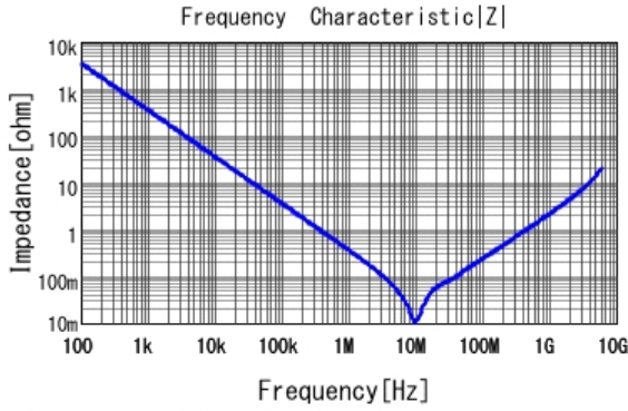
■ GRM188R71C474MA88 |Z| DCOV, 25degC
