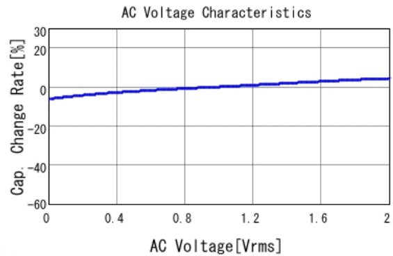
■ GRM188R71C474MA88 C-AC Voltage capchange, DCOV, 25.0d
