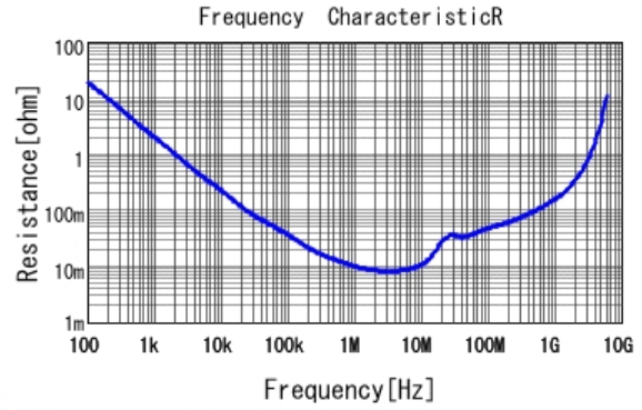
■ GRM188R71C474MA88 R DCOV, 25degC
