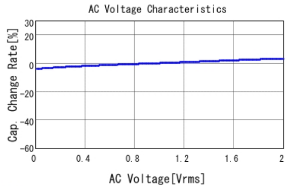
■ GRM188R71C154KA01 C-AC Voltage capchange, DCOV, 25.0d
