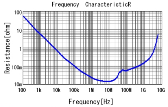
■ GRM188R71C154KA01 R DCOV, 25degC
