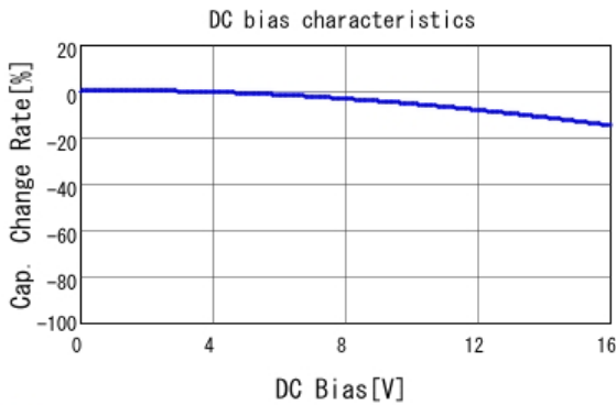
■ GRM188R71C154KA01 C-DC bias capchange, 25.0degC, AC1.
