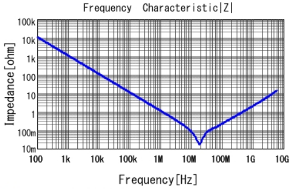
■ GRM188R71C154KA01 |Z| DCOV, 25degC
