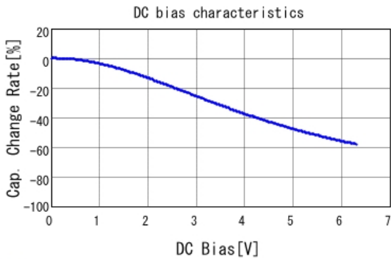
■ GRM188R60J106ME84 C-DC bias capchange, 25.0degC, ACO.
