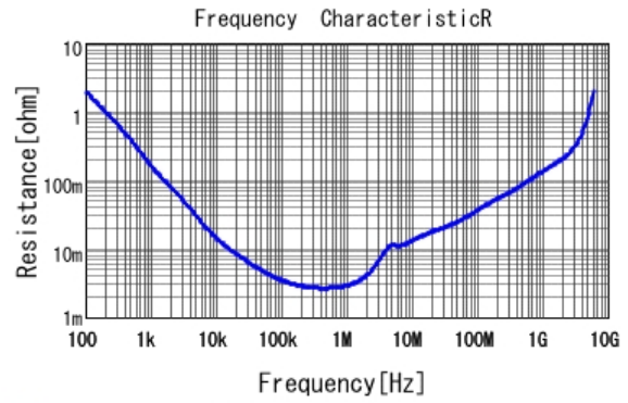
■ GRM188R60J106ME84 R DCOV, 25degC
