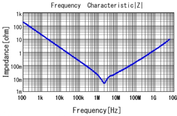
■ GRM188R60J106ME84 |Z| DCOV, 25degC
