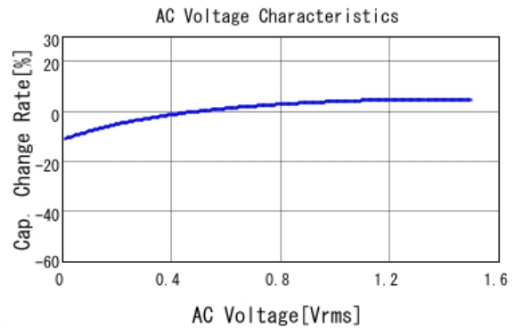
■ GRM188R60J106ME84 C-AC Voltage capchange, DCOV, 25.0d
