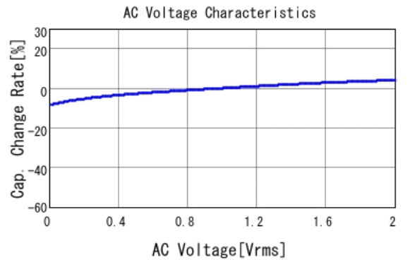
■ GRM188R60J105KA01 C-AC Voltage capchange, DCOV, 25.0d
