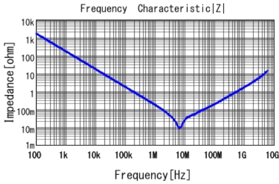
■ GRM188R60J105KA01 |Z| DCOV, 25degC
