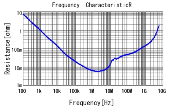
■ GRM188R60J105KA01 R DCOV, 25degC
