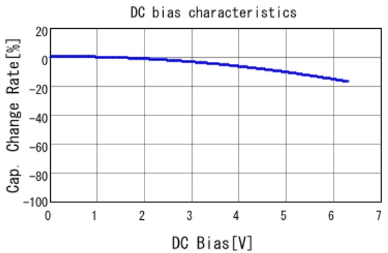
■ GRM188R60J105KA01 C-DC bias capchange, 25.0degC, AC1.
