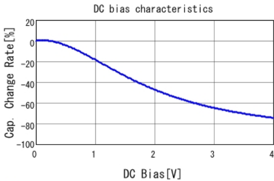
■ GRM188R60G476ME15 C-DC bias capchange, 25.0degC, ACO.
