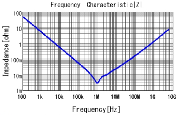
■ GRM188R60G476ME15 |Z| DCOV, 25degC
