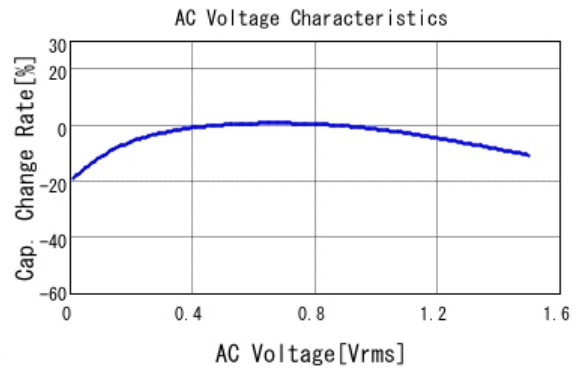
■ GRM188R60G476ME15 C-AC Voltage capchange, DCOV, 25.0d
