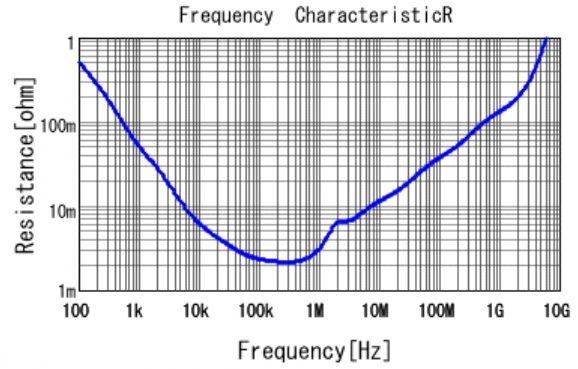
■ GRM188R60G476ME15 R DCOV, 25degC
